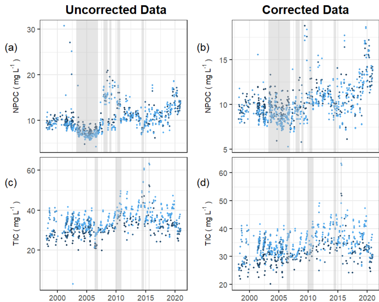
Fig. 1 Time series for NPOC (a, b) and TIC (c, d) illustrating the effect of raw data corrections on temporal dynamics. Grey shaded areas indicate affected time periods.
