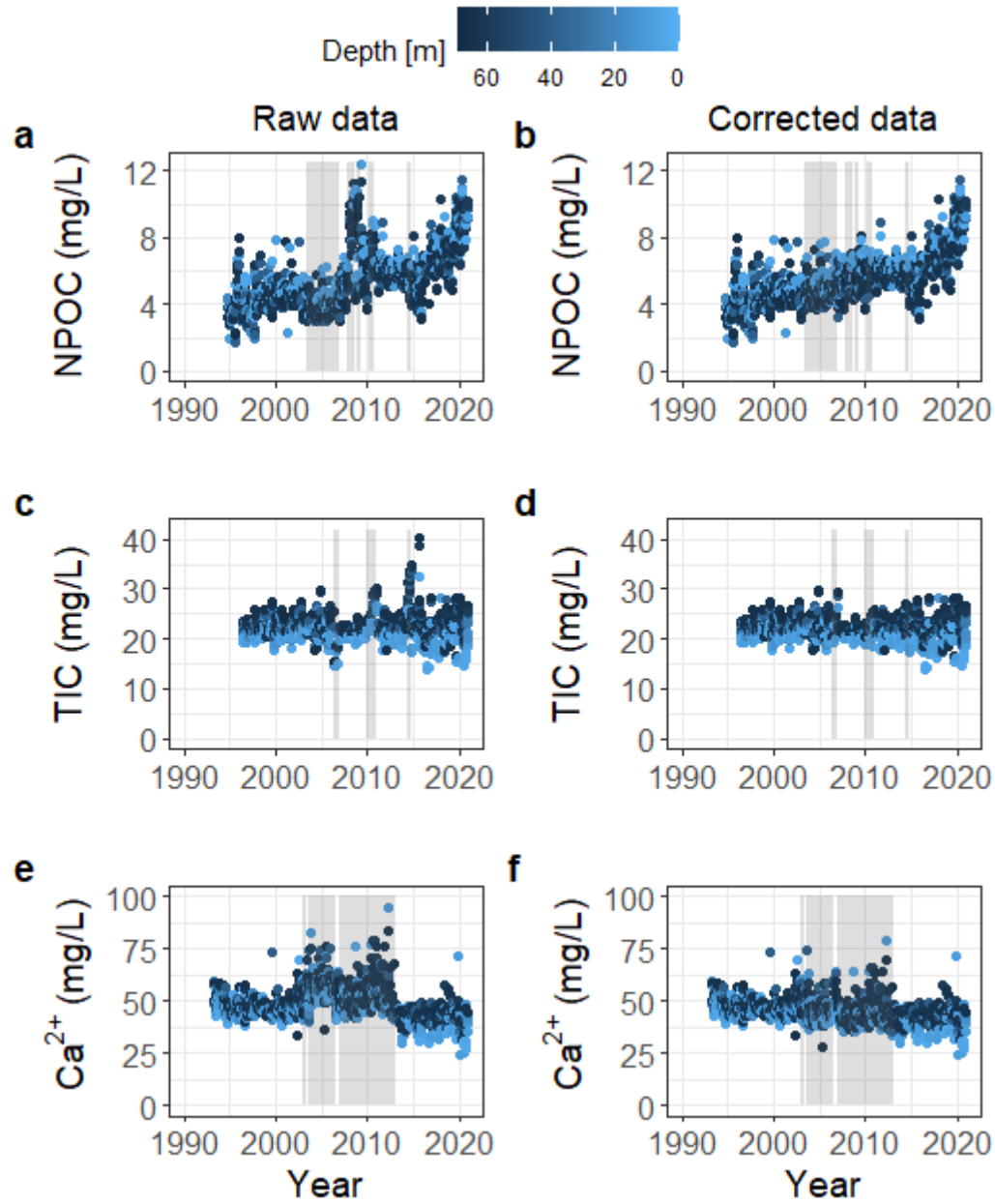
Fig. 1 Time series for NPOC (A, B), TIC (C, D) and spectrophotometrically determined calcium concentrations (E, F), illustrating the effect of raw data corrections on temporal dynamics. Coloured areas indicate affected time periods.
